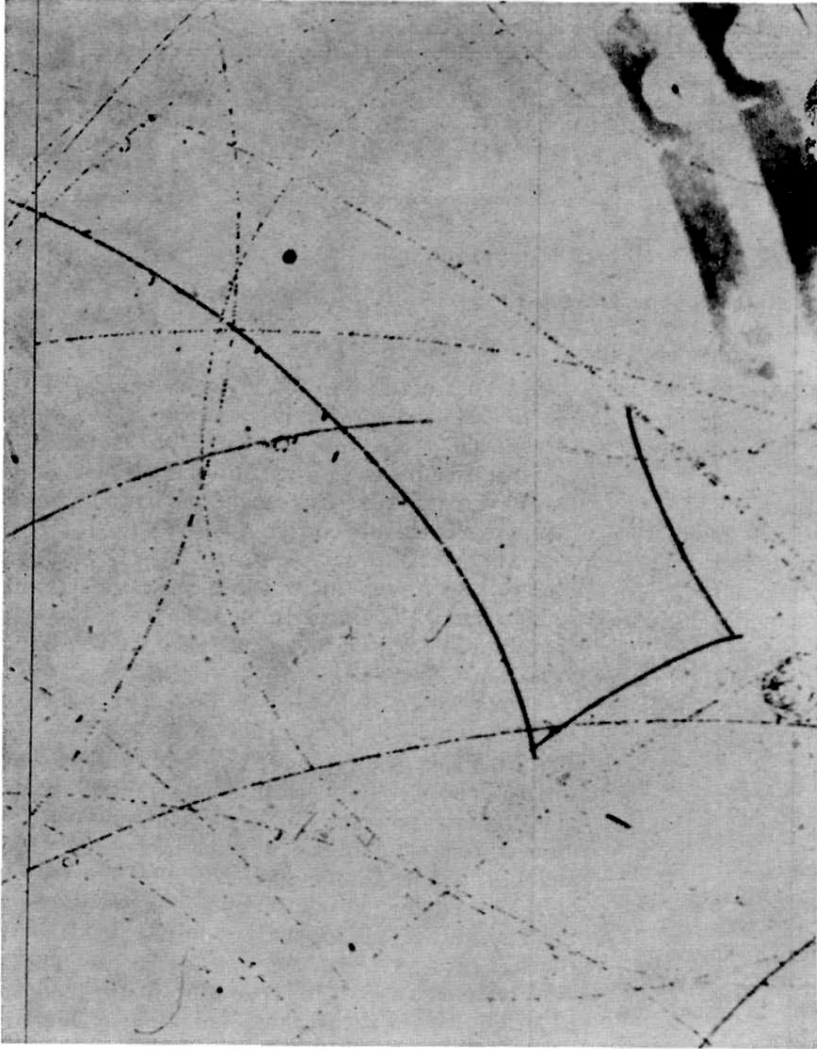
FIG. 3. An example of two successive (d\mu)^+ fusion events in liquid hydrogen. Note the gaps between the stopping muon and the first rejuvenated muon and between the first and second rejuvenated muons.
