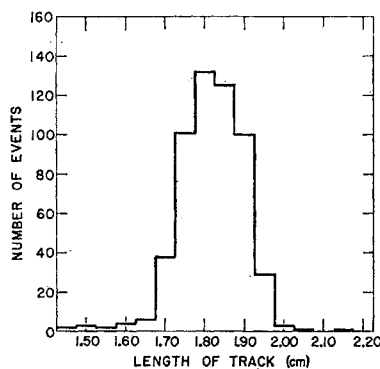
FIG. 6. Range distribution of rejuvenated muons from the (p\mu d)^+ fusion reaction in run \text{H}_2 (pure hydrogen containing 22 ppm \text{D}_2 ).
