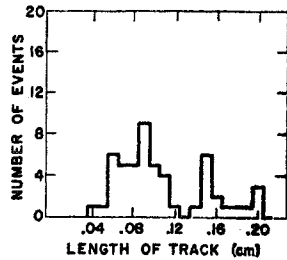
FIG. 9. Range distribution of recoil protons from the (d\mu d)^+ fusion reaction in run D_2I (deuterium containing 1.2% H_2 and <5 \times 10^{-6} parts of air) which did not have an associated decay electron.
