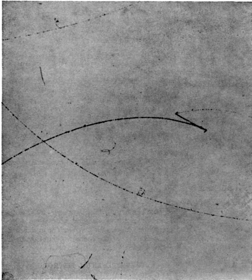
FIG. 5. An example of three successive fusions of the type (d\mu d)^+ \rightarrow p+l+\mu^- , (d\mu p)^+ \rightarrow \text{He}^3+\mu^- , (d\mu d)^+ \rightarrow p+l+\mu^- .
