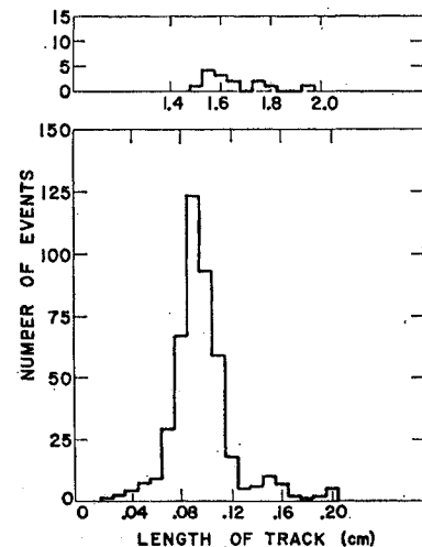
FIG. 8. Range distribution of events in run D 2 I (deuterium containing 1.2% H 2 and <5 \times 10^{-5} parts of air). The upper section shows the rejuvenated muons from the (p\mu d)^+ fusion reaction, and the lower section the recoil protons from the (d\mu d)^+ fusion reaction.
